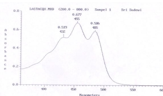
Figure 6. Ultraviolet spectrum (CHCl 3 ) of the isolated compound
