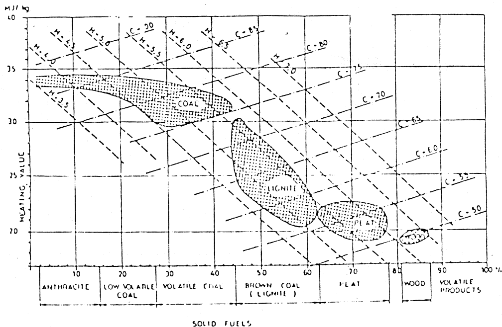
Gambar 3. Comparison of solid fuels. (Kalmari, 1982a)
