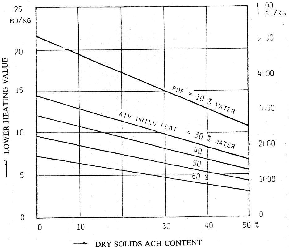
Gambar 4. Lower heating value of peat fuels (Myreen, 1983).
