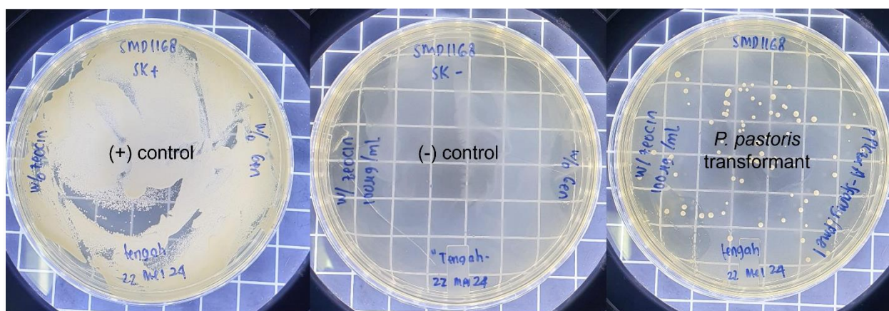
Figure S2. Transformant of P. pastoris SMD1168 by pPICZαA-sfamy-mutant.
