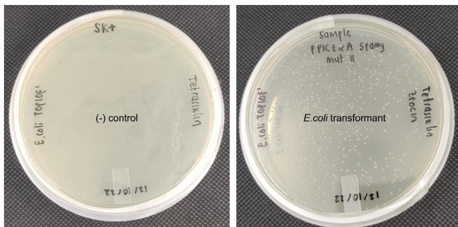
Figure S1. pPICZαA-Sfamy-mutant in E. coli TOP10 clone, negative control ( E. coli TOP10 without plasmid) and transformant colony in a Zeocin-resistant plate.
