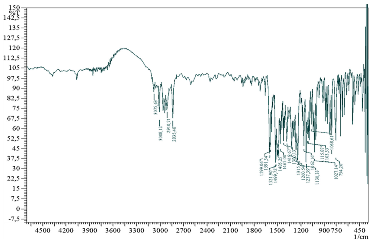
Fig S13. FTIR spectrum of 4d
