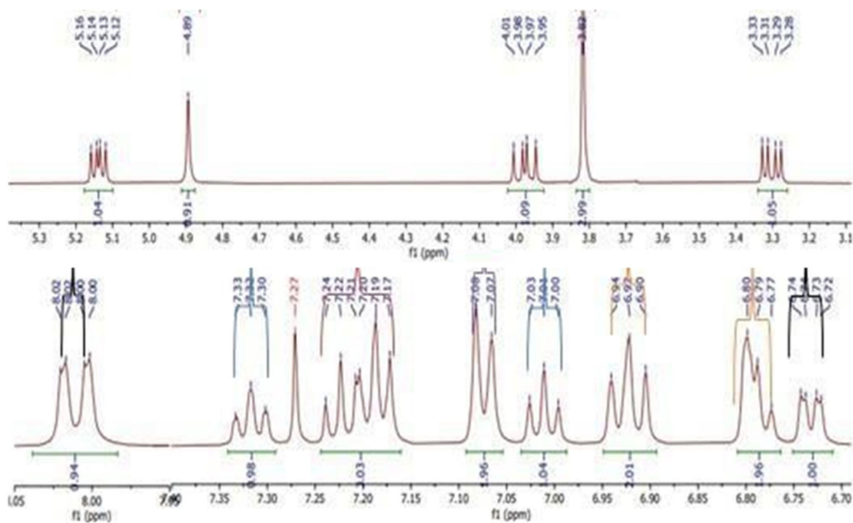
Fig S12. ^1\text{H} -NMR spectrum of 4c
