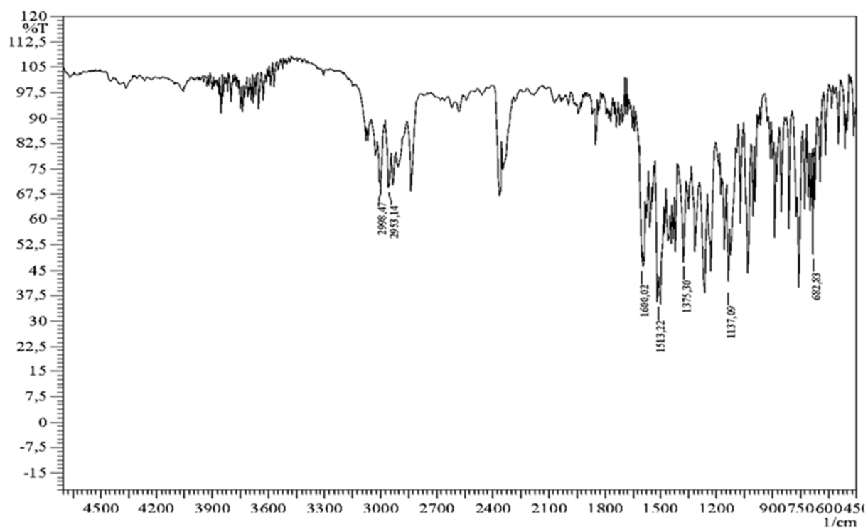
Fig S6. FTIR spectrum of 4b
