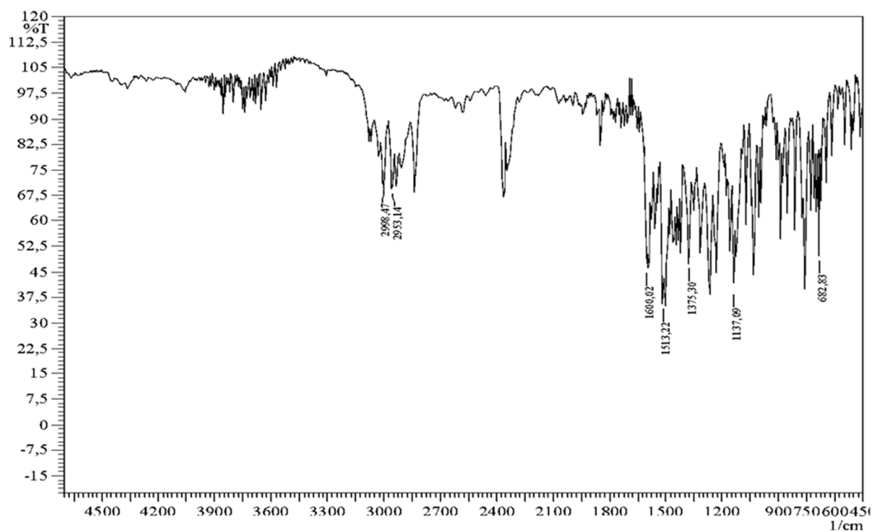
Fig S10. FTIR spectrum of 4c
