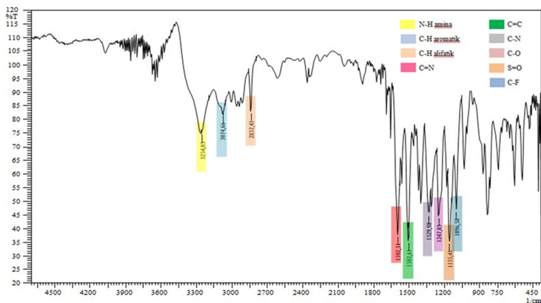
Fig S16. FTIR spectrum of 4e
