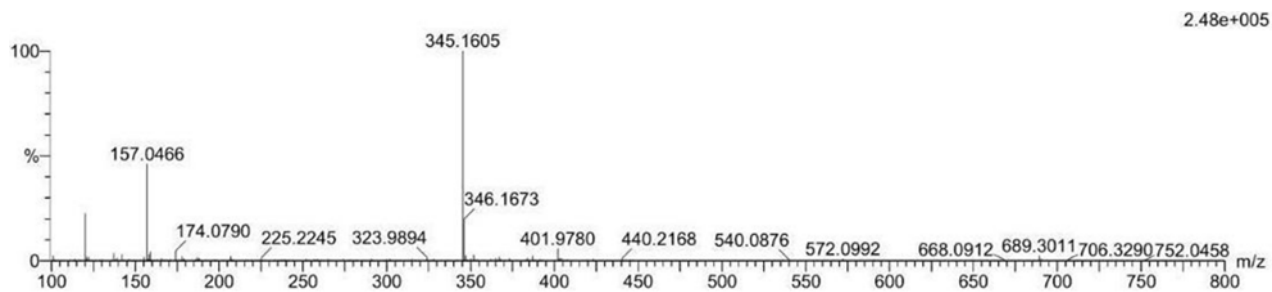
Fig S11. HRMS spectrum of 4c
