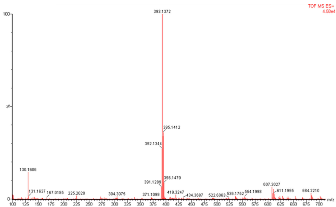
Fig S14. HRMS spectrum of 4d
