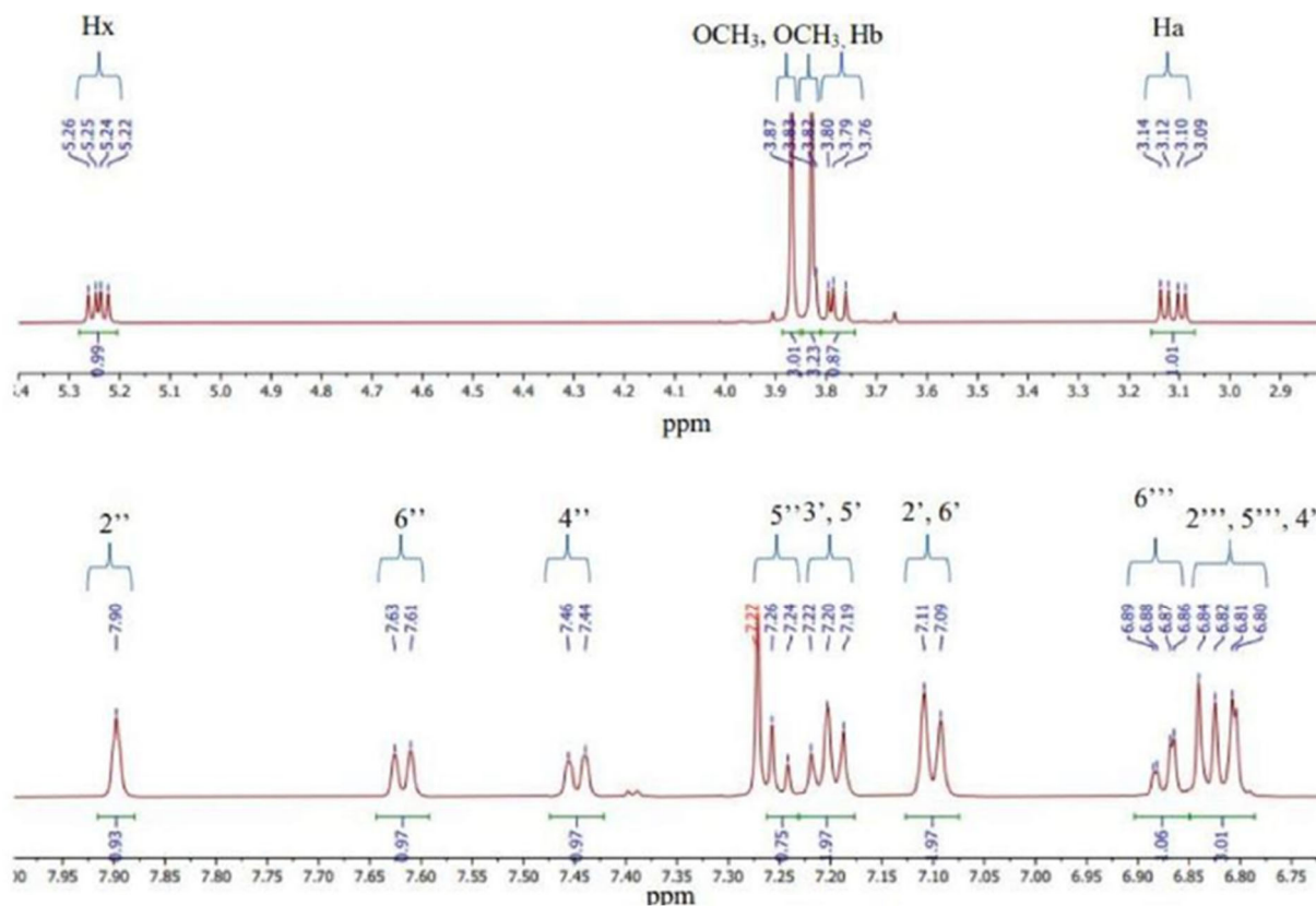
Fig S8. 1 H-NMR spectrum of 4b
