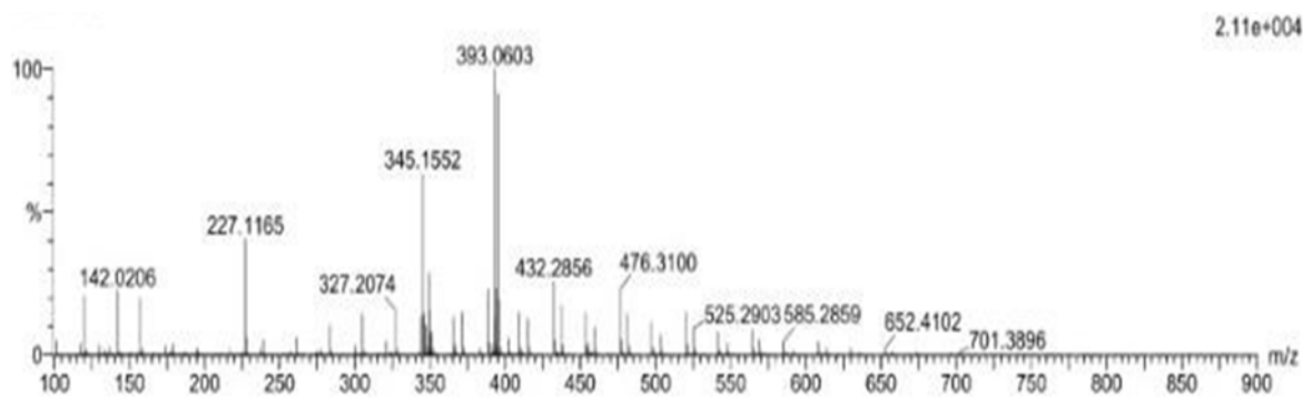
Fig S7. HRMS spectrum of 4b
