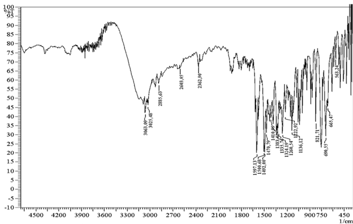
Fig S2. FTIR spectrum of 4a
