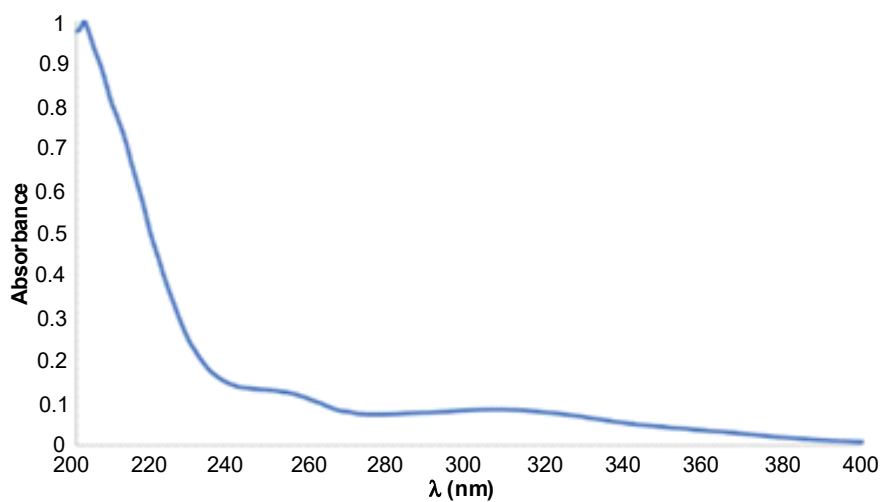
Fig S1. UV-vis spectrum of 4a
