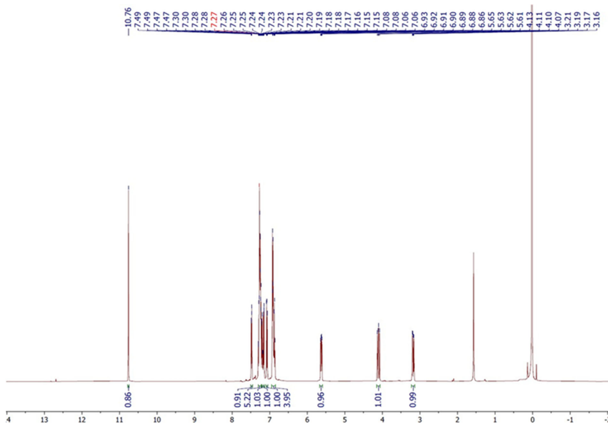
Fig S4. 1 H-NMR spectrum of 4a
