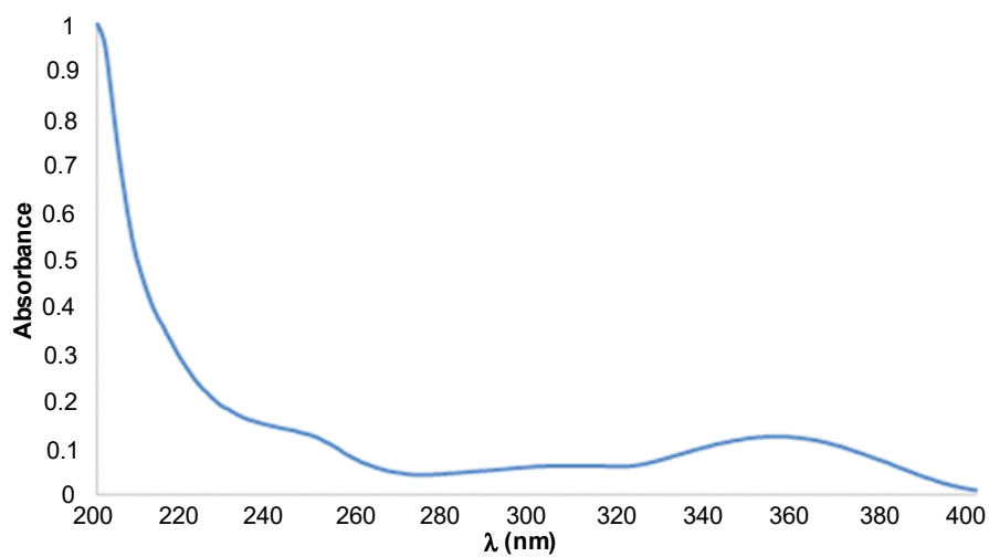
Fig S5. UV-vis spectrum of 4b
