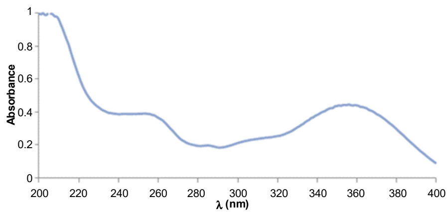
Fig S9. UV-vis spectrum of 4c
