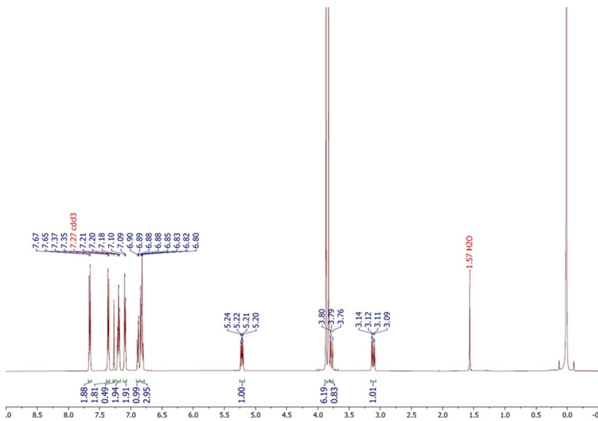
Fig S15. 1 H-NMR spectrum of 4d
