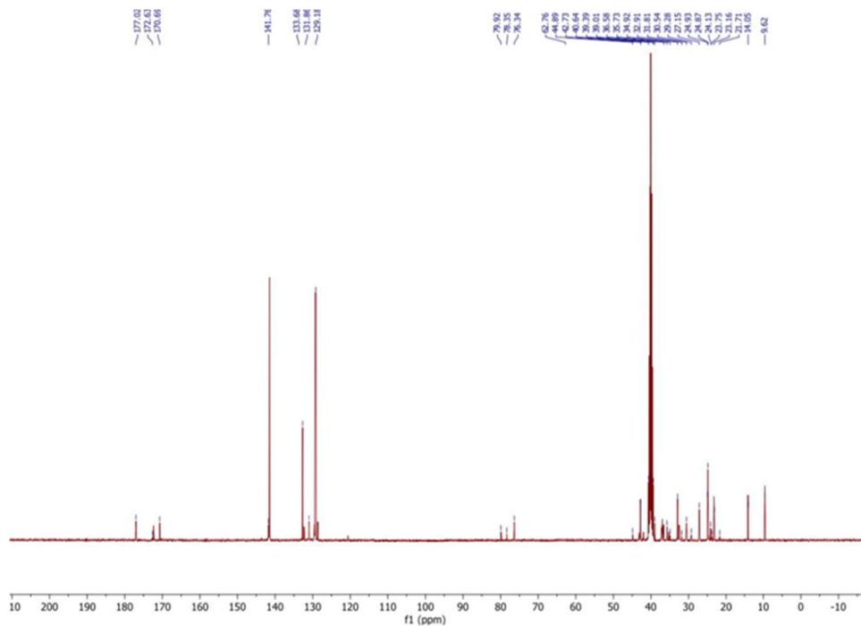
Fig S3. 13 C-NMR spectrum of compound A1
