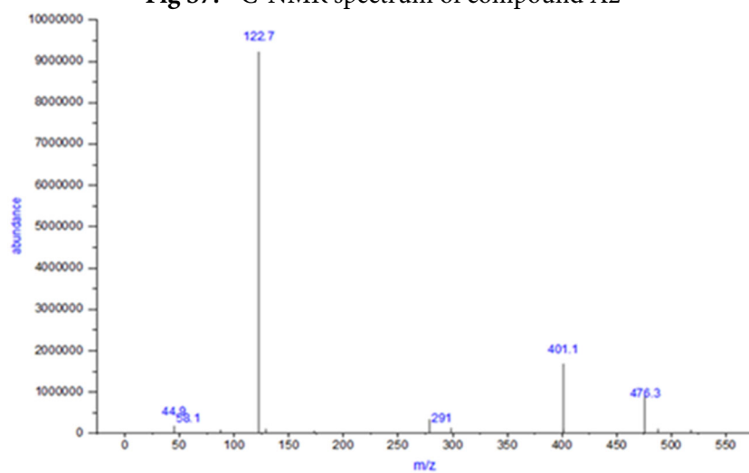
Fig S8. Mass spectrum of compound A2
