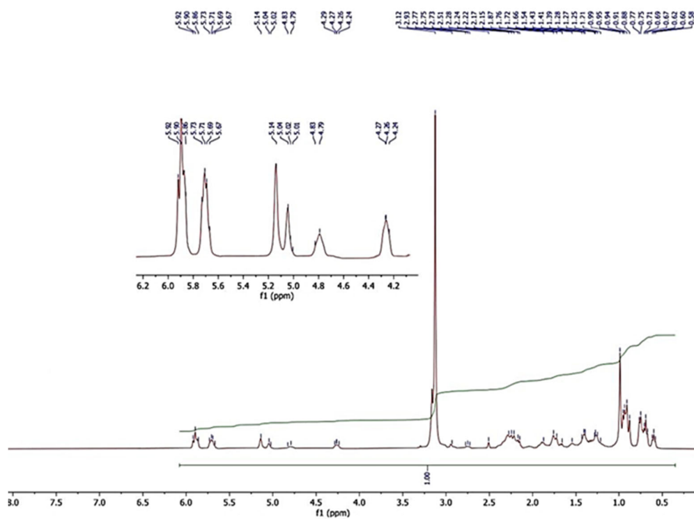
Fig S6. 1 H-NMR spectrum of compound A2
