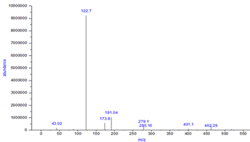
Fig S4. Mass spectrum of compound A1
