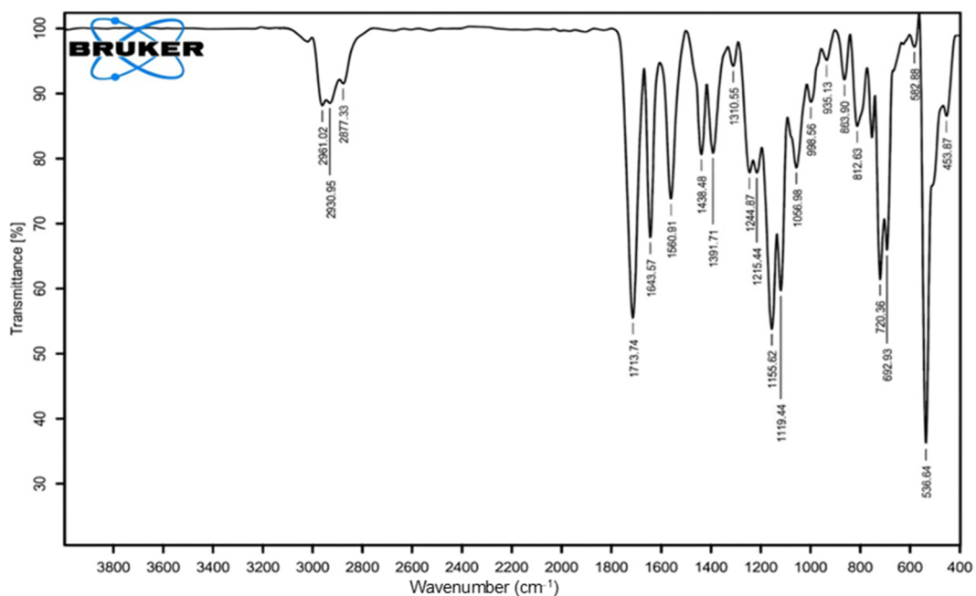
Fig S5. FTIR spectrum of compound A2
