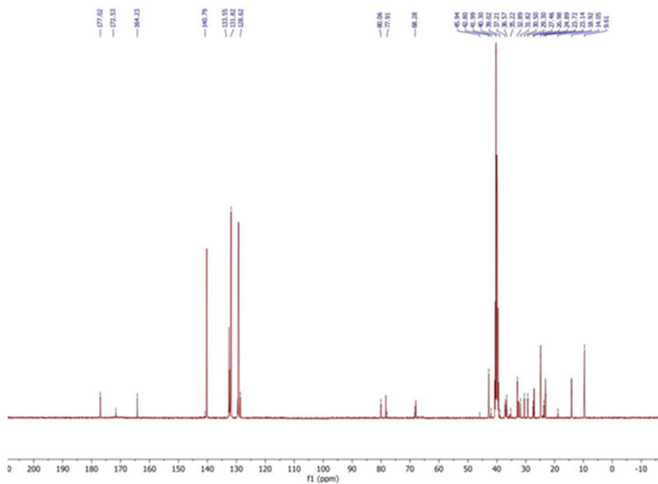
Fig S7. ^{13}\text{C} -NMR spectrum of compound A2
