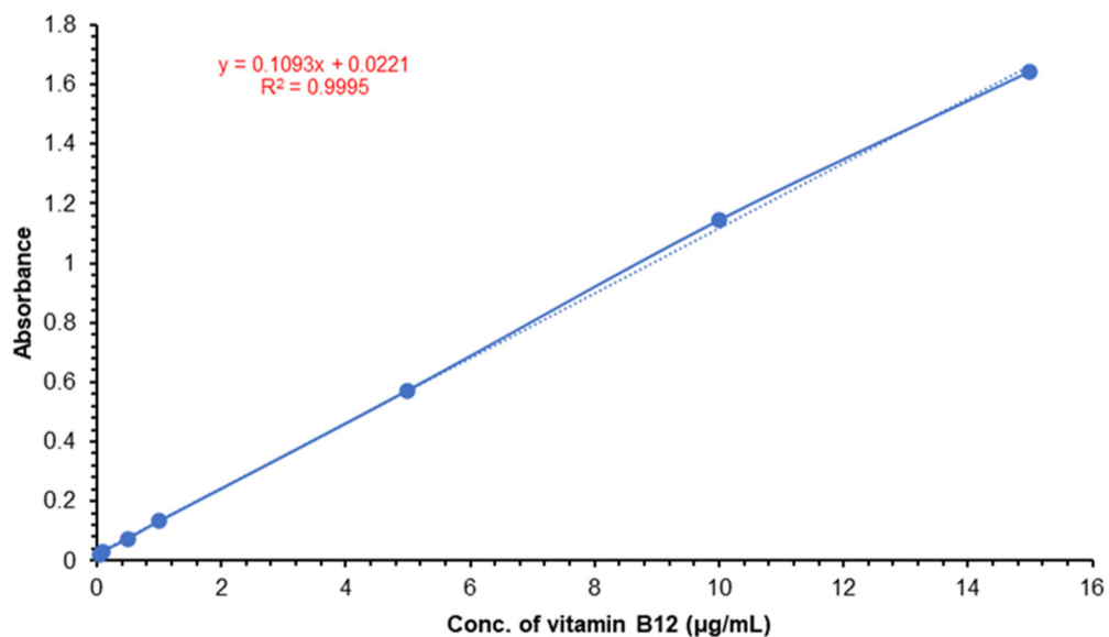
Fig S5. Calibration curve of vitamin B12 after extraction by GO
