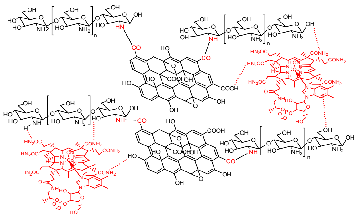
Fig S3. Hypotheses for the adsorption of VB12 on the surface of the GO/CTS composite
