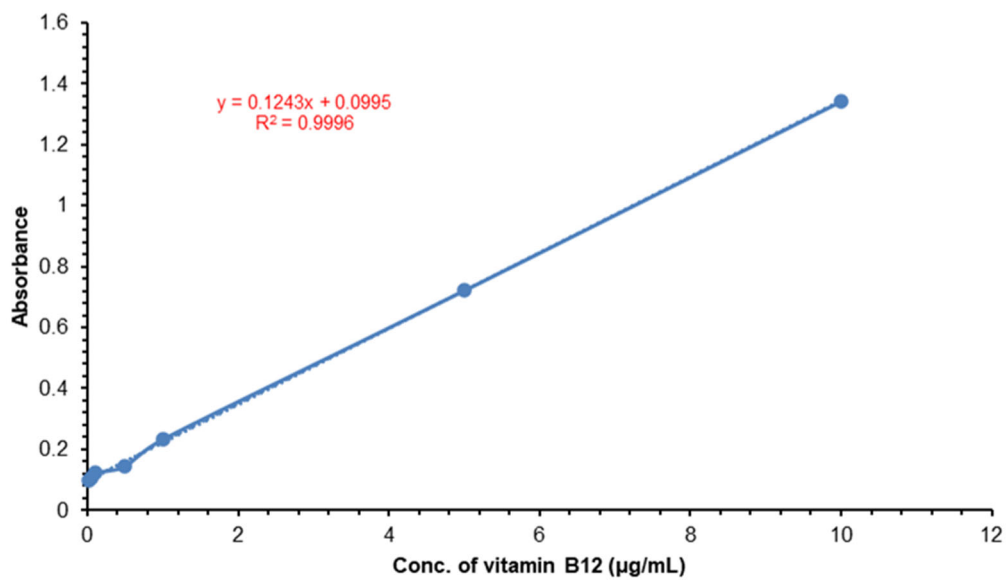
Fig S7. Calibration curve of vitamin B12 after extraction using GO/CTS
