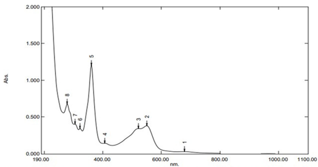
Fig S4. Absorption spectrum of vitamin B12
