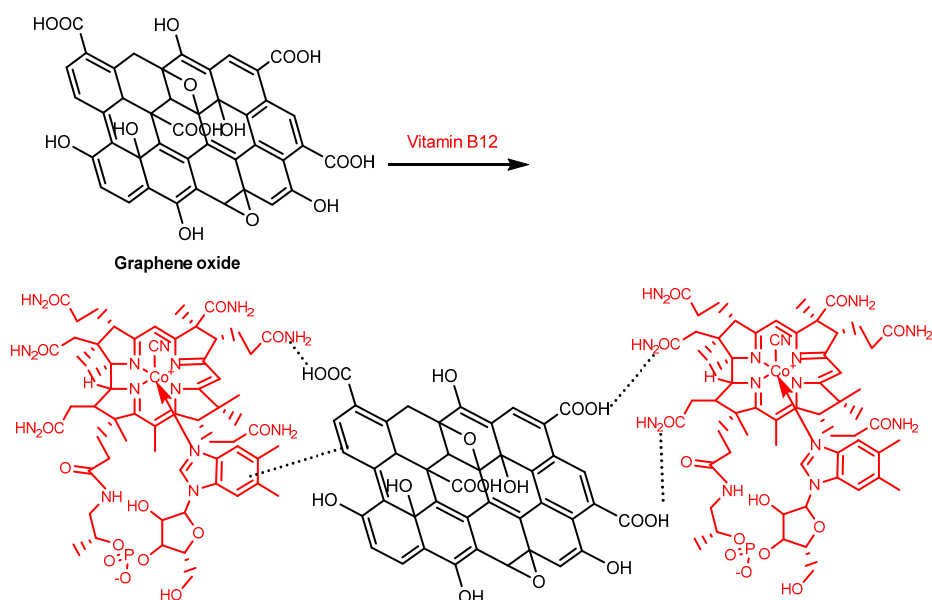
Fig S1. Hypotheses for the adsorption of VB12 on the surface of GO
