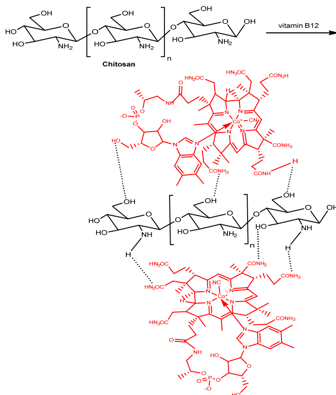
Fig S2. Hypotheses for the adsorption of VB12 on the surface of CTS
