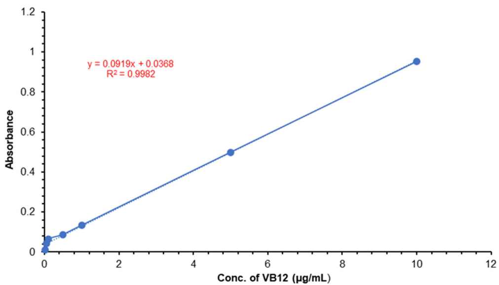
Fig S6. Calibration curve of vitamin B12 after extraction by CTS
