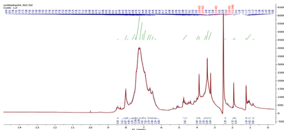
Fig S1. 1 H-NMR spectrum of ligand (4-FADPD)
