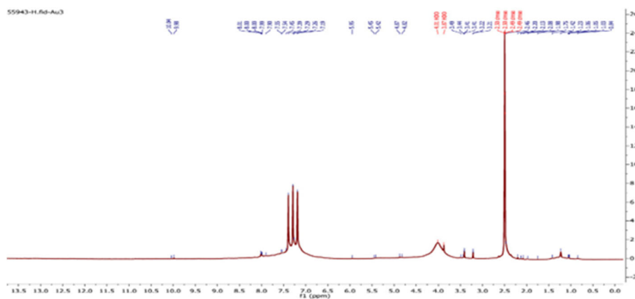
Fig S4. 1 H-NMR spectrum of [Au(L)Cl]Cl 2 ·H 2 O complex
