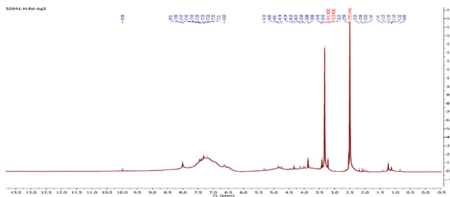
Fig S3. 1 H-NMR spectrum of [Ag(L)H 2 O]NO 3 complex
