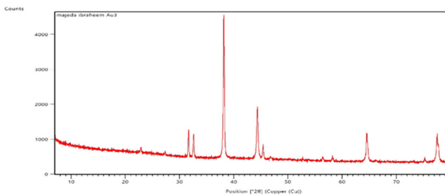
Fig S16. XRD of [\text{Au}(\text{L})\text{Cl}]\text{Cl}_2 \cdot \text{H}_2\text{O} complex
