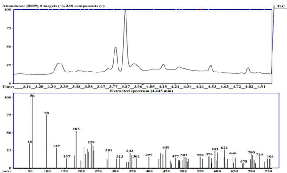
Fig S6. Mass spectrum of the [Au(L)Cl]Cl 2 ·H 2 O complex
