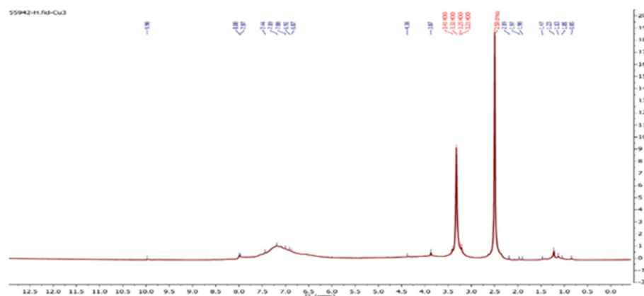
Fig S2. 1 H-NMR spectrum of [Cu(L)Cl 2 (H 2 O)] complex
