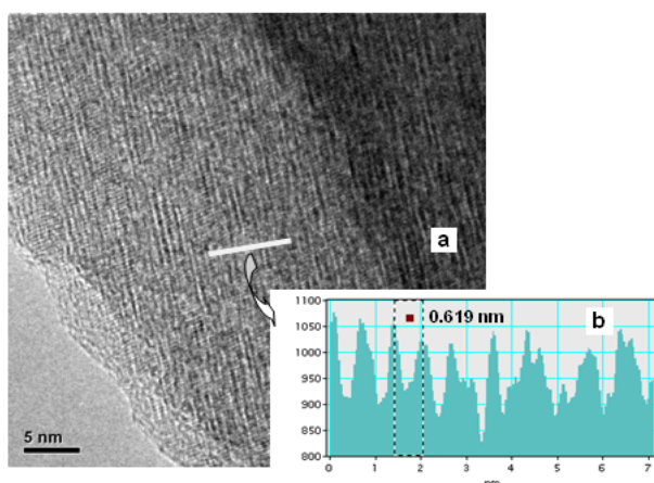
Fig 6. (a). HRTEM image and (b). electron diffraction spectra of TiO_2(B) (the powder obtained by heat treatment of protonic lepidocrocite titanate for 2 h at 300 °C)
