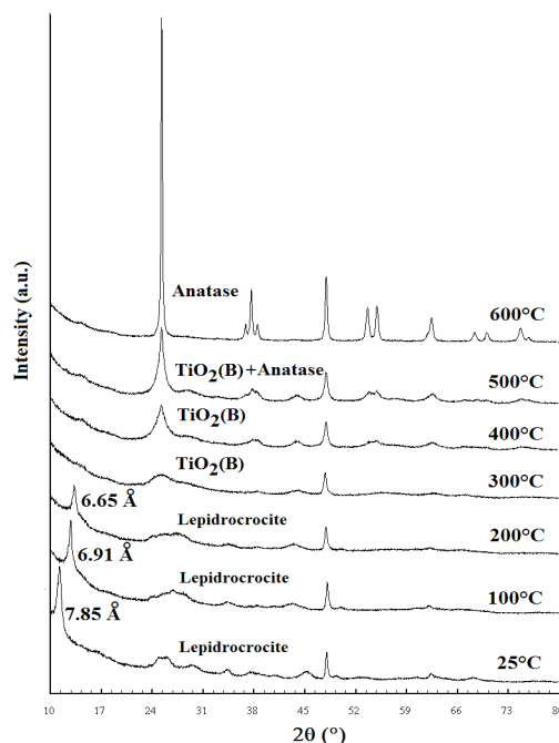
Fig 4. XRD patterns of samples before and after the heat treatment of \text{H}_{0.54}\text{Ti}_{1.865}\text{O}_4 \cdot 0.5\text{H}_2\text{O}
