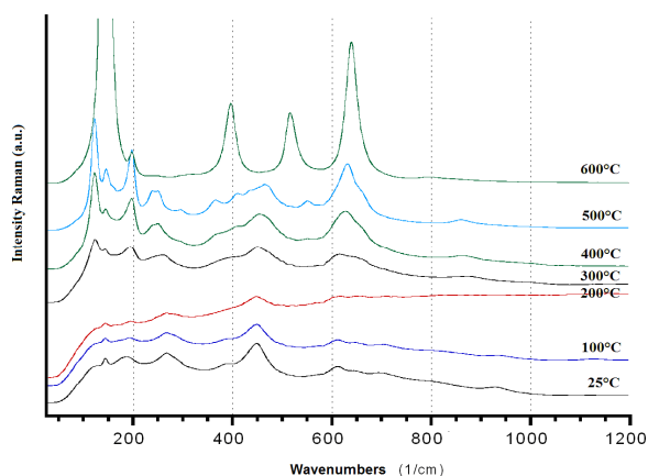
Fig 5. Raman spectra of samples before and after the heat treatment of H_{0.54}Ti_{1.865}O_{4} \cdot 0.5H_2O
