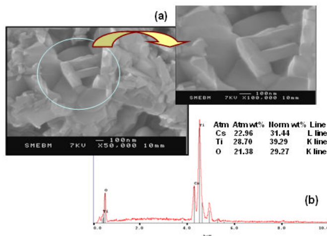
Fig 1. (a). SEM image and (b). EDX of sesium titanate
