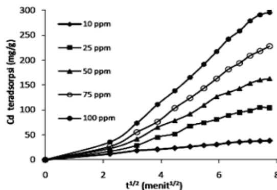
Gambar 14. Kurva hubungan Cd(II) teradsorpsi versus t^{1/2}
