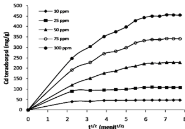
Gambar 15. Kurva hubungan Cd(II) teradsorpsi versus t^{1/2}
