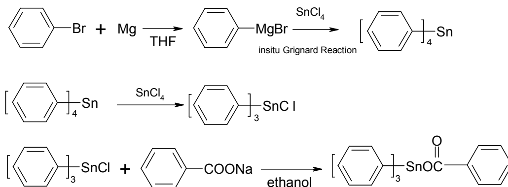
Figure 1. Reaction scheme for synthesizing triphenyltin benzoate
