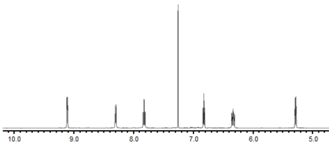
Fig S2. 1 H-NMR spectra of Ir(III) dimer, [\text{Ir}(2,4\text{-F}_2\text{ppy})_2(\mu\text{-Cl})_2]
