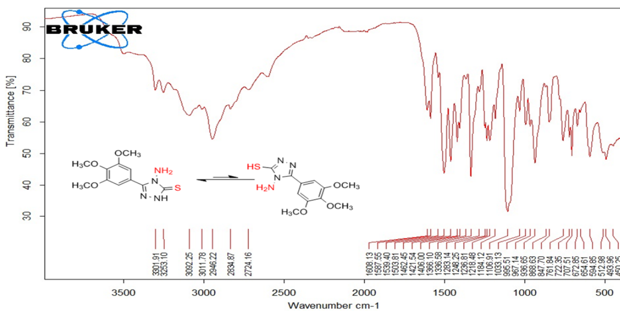
Fig S1. FT-IR spectrum of 4-amino-5-(3,4,5-trimethoxyphenyl)-4H-1,2,4-triazole-3-thione, L
