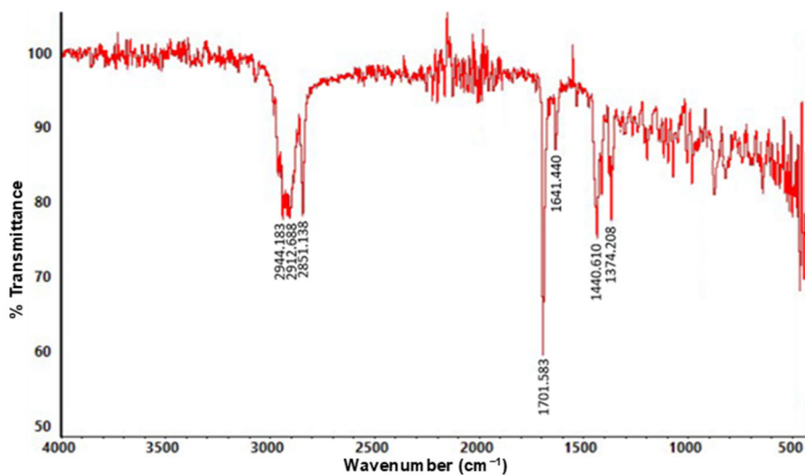
Fig S1. IR spectrum of compound 1
