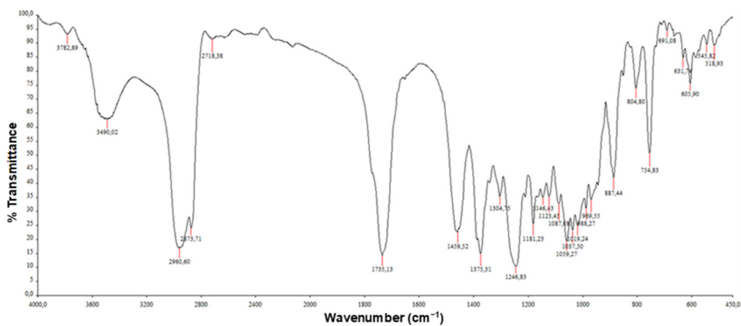
Fig S4. IR spectrum of compound 4
