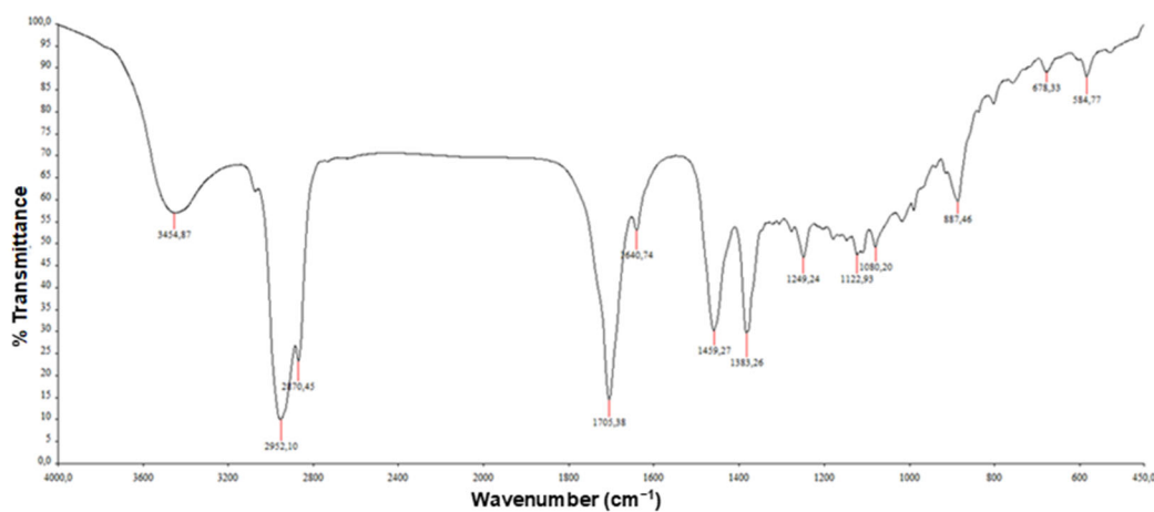
Fig S2. IR spectrum of compound 2
