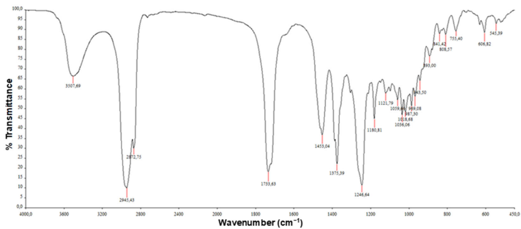
Fig S3. IR spectrum of compound 3
