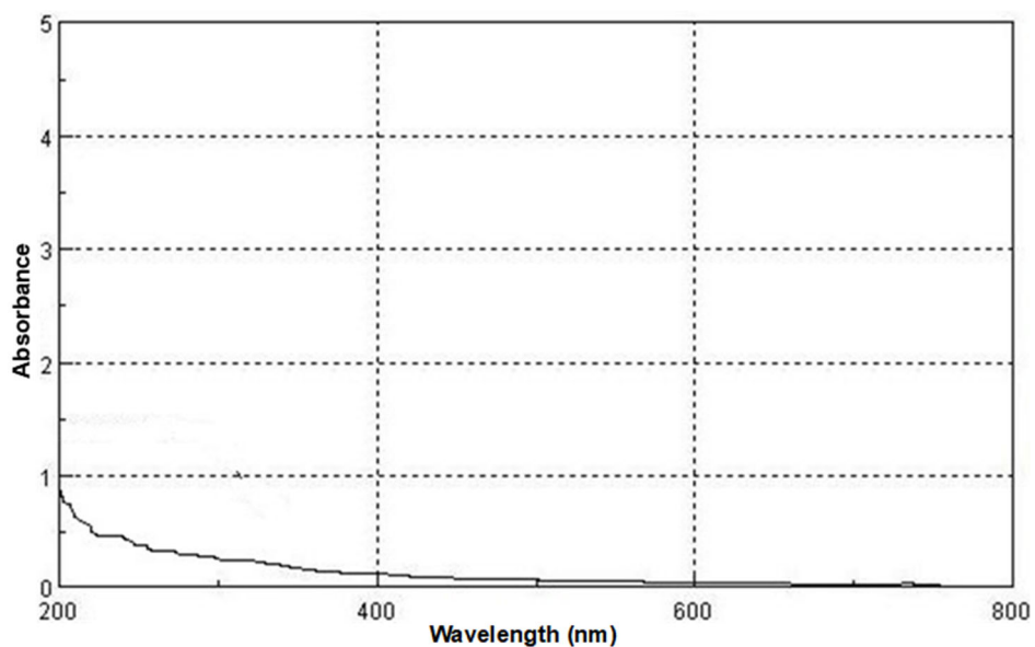
Fig S2. Blank spectrum against distilled water
