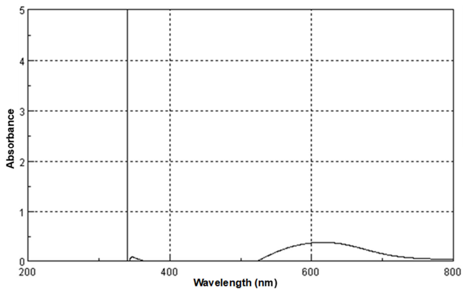
Fig S1. The absorption spectrum of the oxidative coupling product
