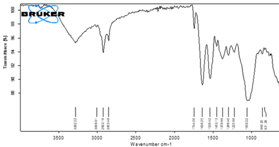
Fig S1. FTIR analysis of ACNPs
