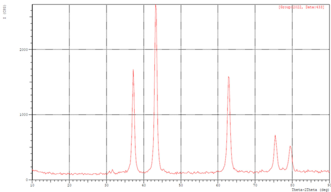
Fig S2. XRD patterns of the ACNPs
