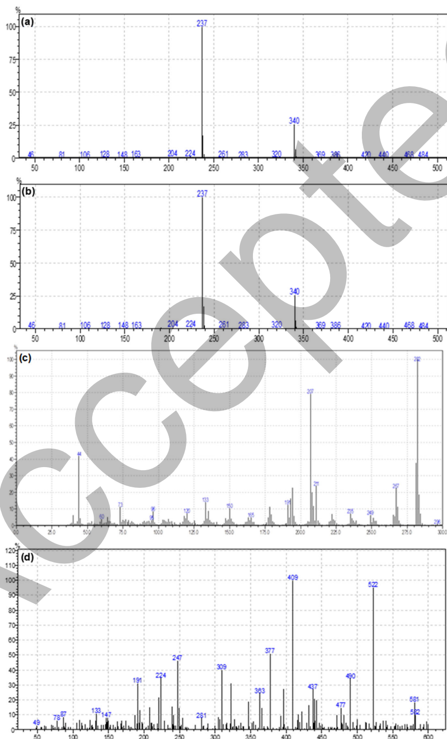
Fig S1. Mass spectrum of (a) A1 derivative, (b) A2 derivative, (c) Schiff base L, and (d) CoL complex
