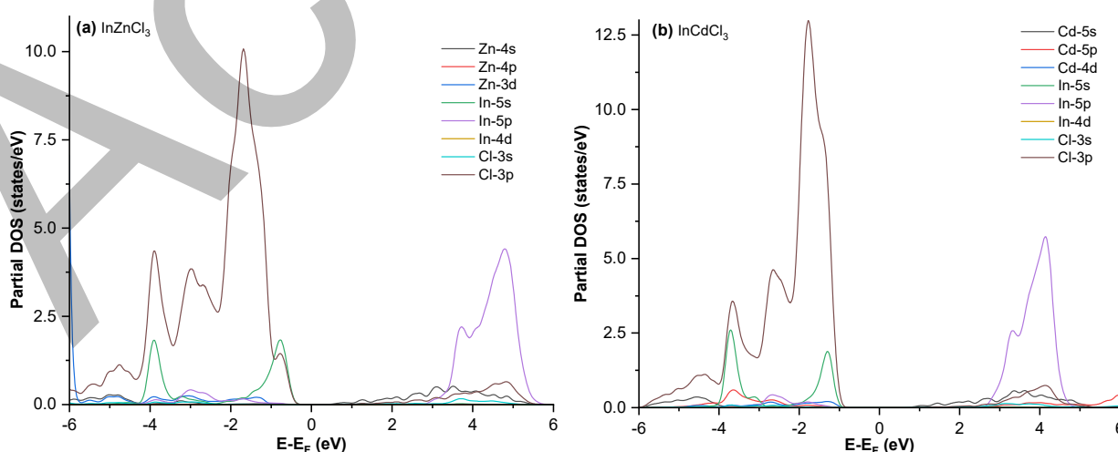
Fig 5. PDOS of cubic (a) InZnCl_3 and (b) InCdCl_3 perovskites
