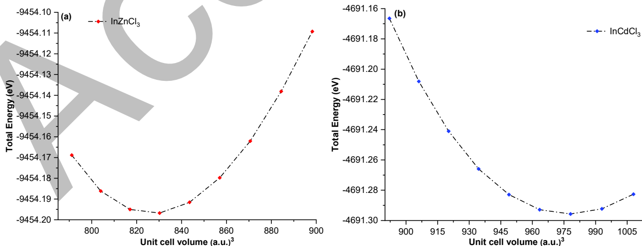
Fig 2. Total energy vs unit cell volume of (a) \text{InZnCl}_3 and (b) \text{InCdCl}_3 perovskites
