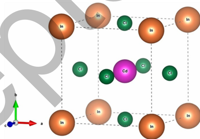
Fig 1. The unit cell structure of cubic \text{InCdCl}_3 perovskite material
