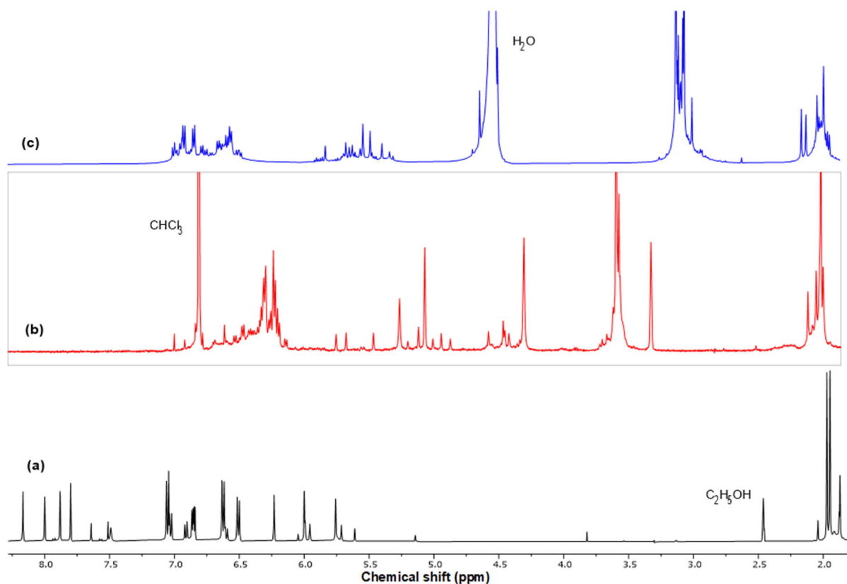
Fig 2. The ^1\text{H-NMR} spectra of (a) C -4-chlorophenylcalix[4]-2-methylresorcinarene, (b) C -4-methoxyphenylcalix[4]-2-methylresorcinarene, and (c) C -4-dimethylaminophenylcalix[4]-2-methylresorcinarene
