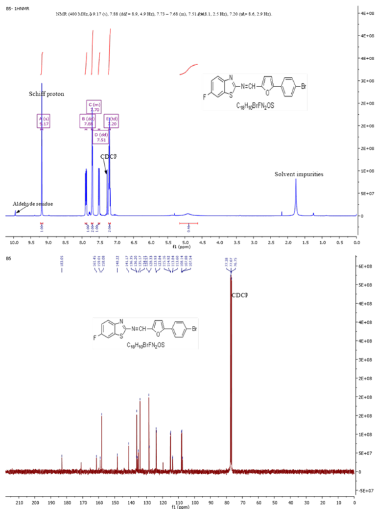
Fig S3. The NMR (proton and carbon) spectra of B1–B5
