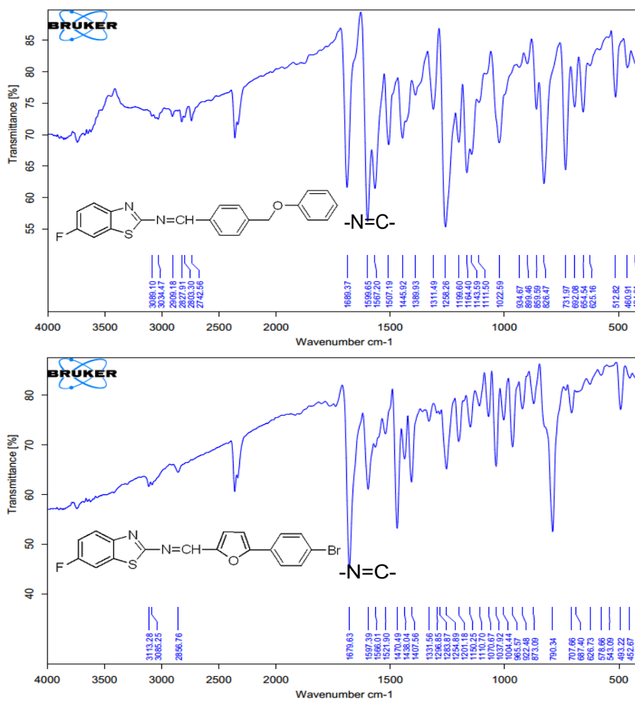
Fig S1. The IR spectra of B1–B5
