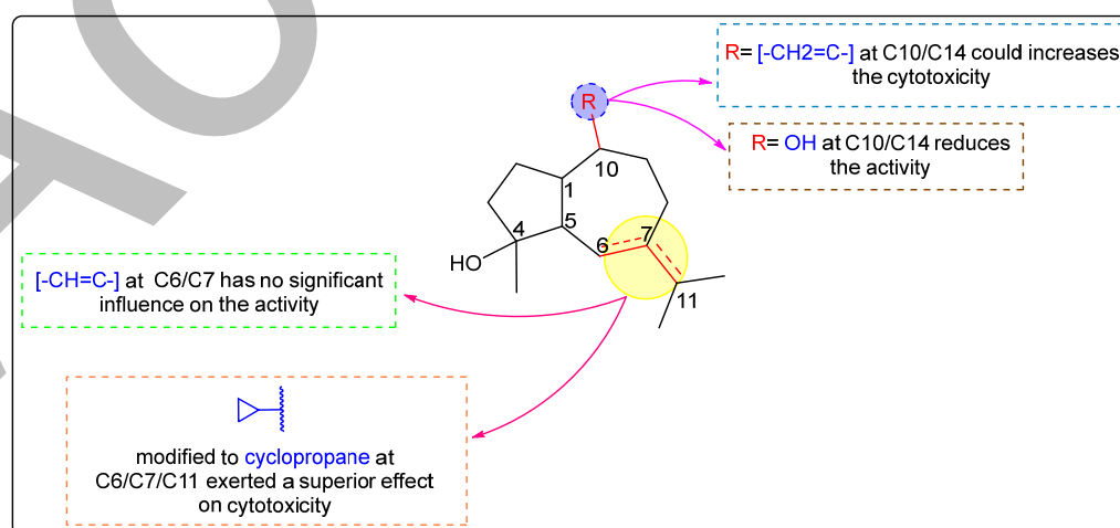
Fig 4. The structure-activity relationship of sesquiterpenoids 1–3
