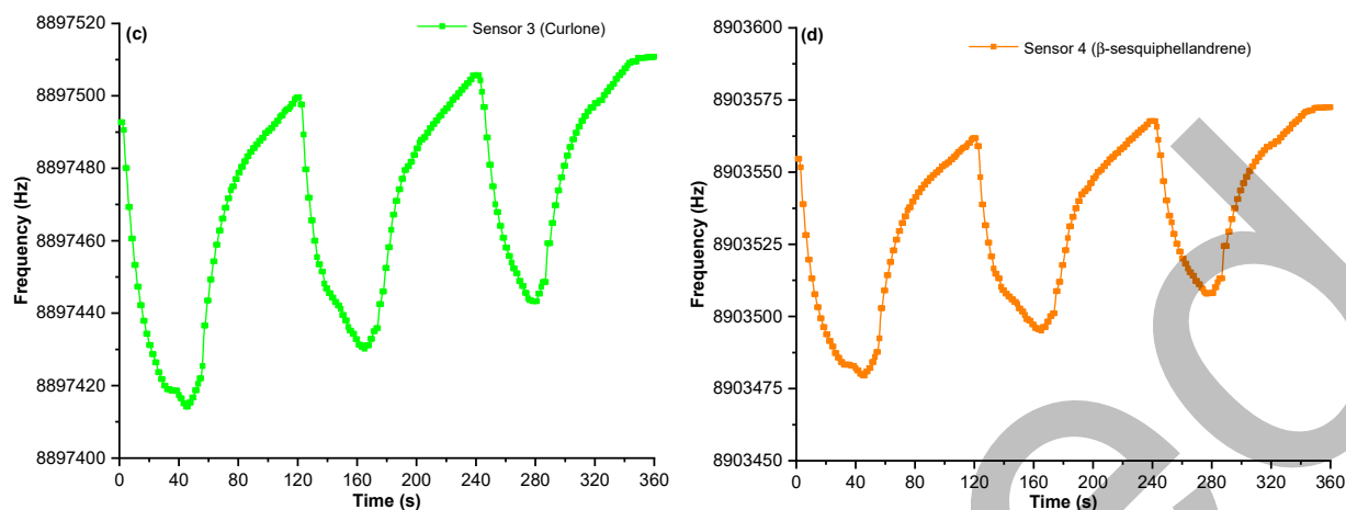
Fig 5. The Typical response of the MIP-QCM sensor array towards turmeric odor exposure at the sample of TEO i : (a) sensor 1 ( \alpha -curcumene), (b) sensor 2 (ar-turmerone), (c) sensor 3 (curlone), (d) sensor 4 ( \beta -sesquiphellandrene)
