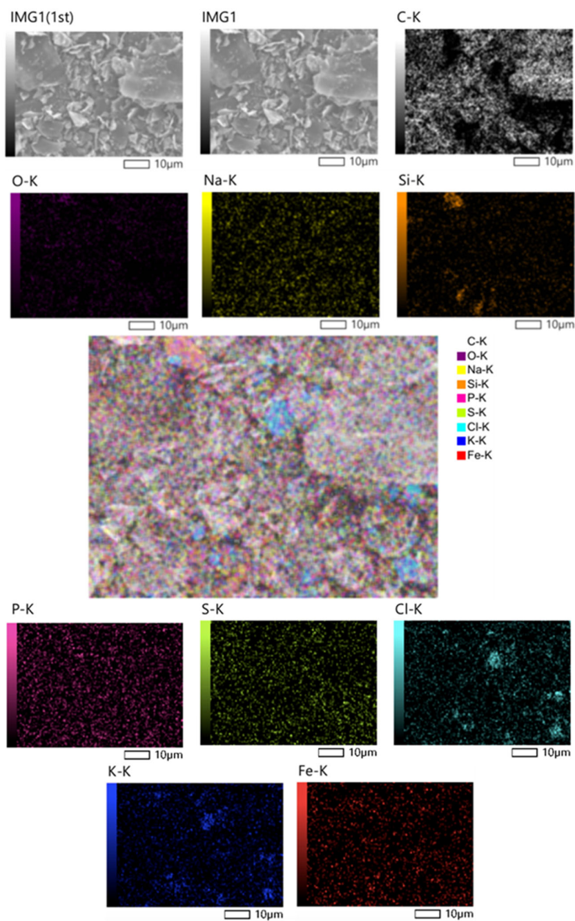
Fig S3. Maps of elements onto biochar surface
