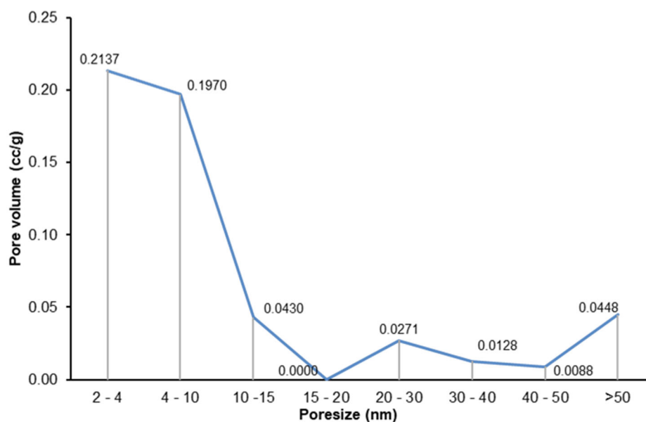
Fig S1. Pore size distribution of biochar by BET analysis
