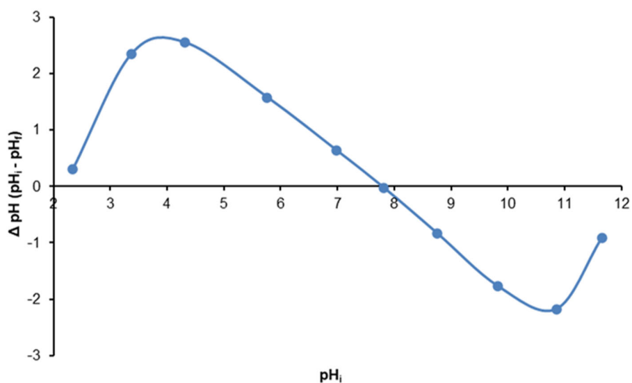
Fig S2. Point of zero charge determination for biochar
