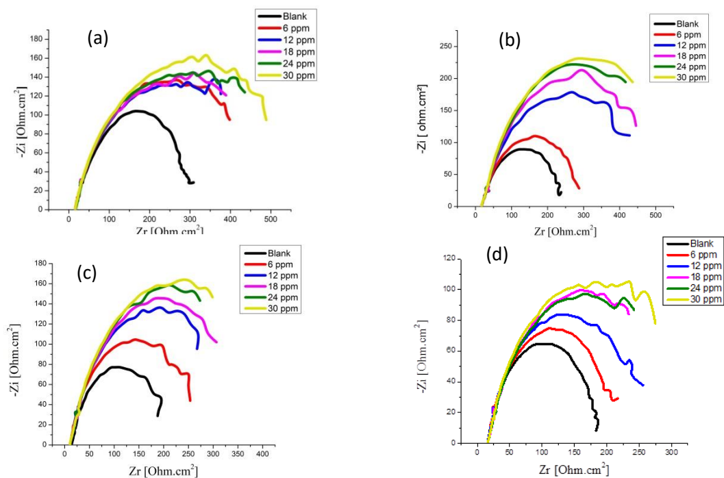
Nyquist curves of N,O -CMCs at (a) 25, (b) 35, (c) 45, (d) 55 °C
