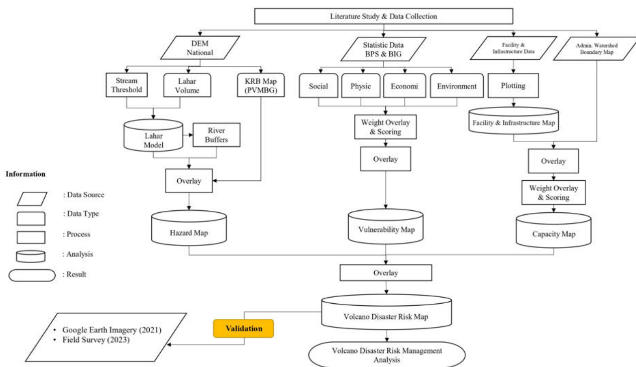
Figure 2. Research Methodology
