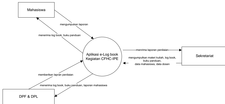
Gambar 1. Context Diagram
