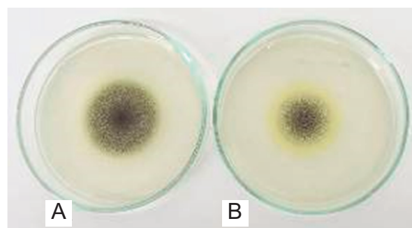
Figure 1. Aspergillus niger isolates after treated with sulfuryl fluoride; control (A), treated with sulfuryl fluoride at concentration of 30 g/m 3 for 24 hours (B)
