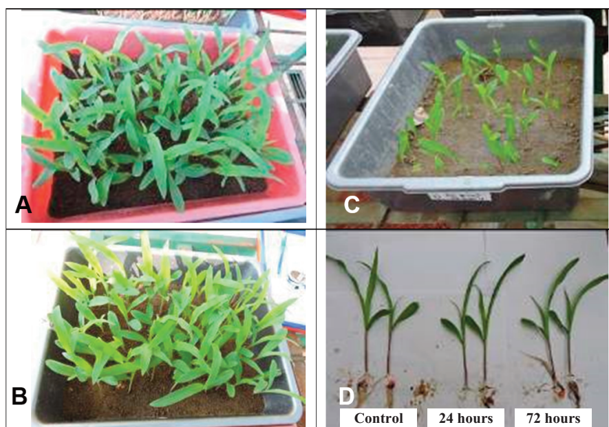
Figure 2. Corn seeds after 7 days; control (A), treated with sulfuryl fluoride at concentration of 30 g/m 3 for 24 hours (B), treated with sulfuryl fluoride at concentration of 50 g/m 3 for 72 hours (C), physical growth of treated and untreated seeds (D)
