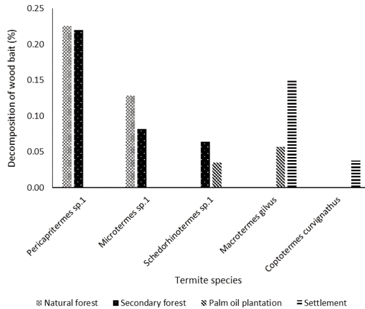
Figure 2. Percentage of decomposition on wood baits of termites in different land use
