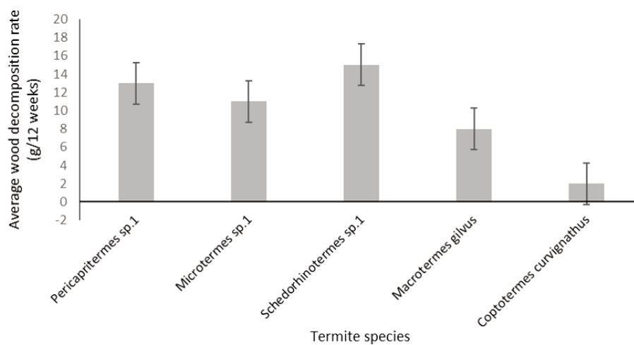
Figure 3. Mean decomposition rate of each termite species found on wood baits
