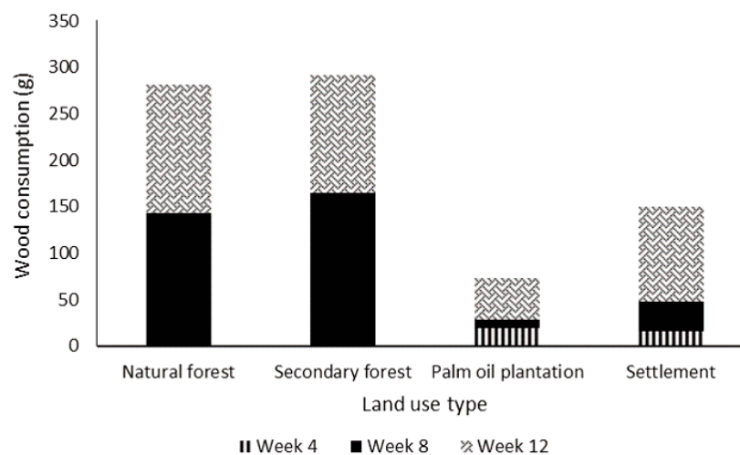
Figure 1. Wood consumption by termites at different observation periods
