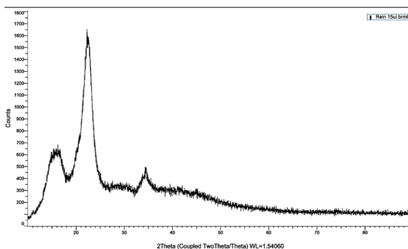
Fig. 6: XRD diffractogram on Sample Run 15
