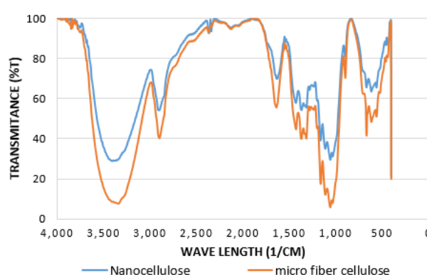
Fig. 5: FTIR spectrum of Sample Run 15
