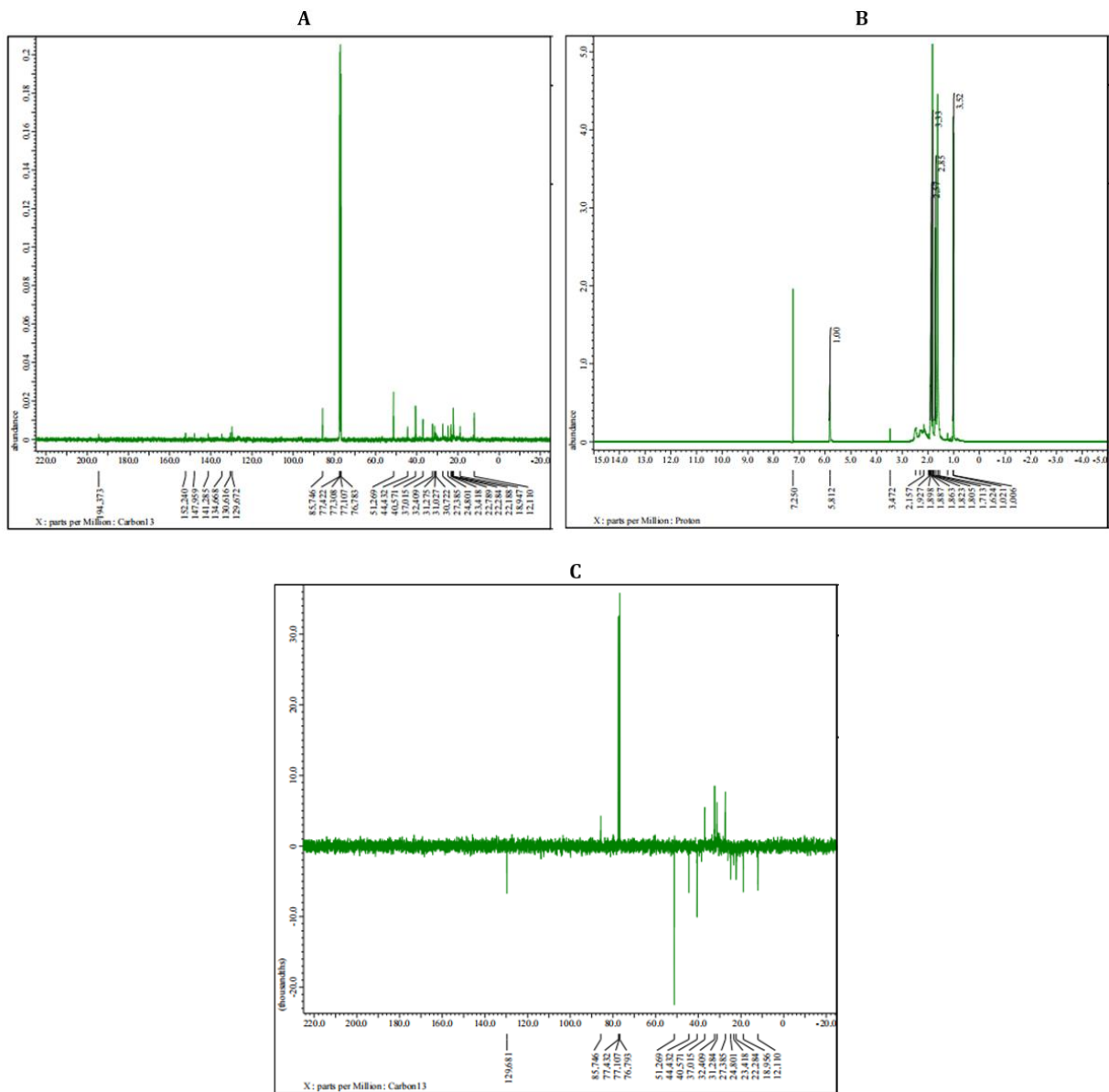
Supplementary Figure 2. NMR analysis of isolate FLE.A2. Analysis of ^{13}\text{C} -NMR ( A ), ^1\text{H} -NMR ( B ), and APT-NMR ( C )
