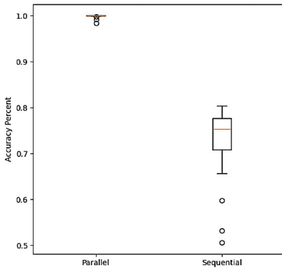
Figure 4. Comparison t-test parallel of sequential and parallel configuration.
