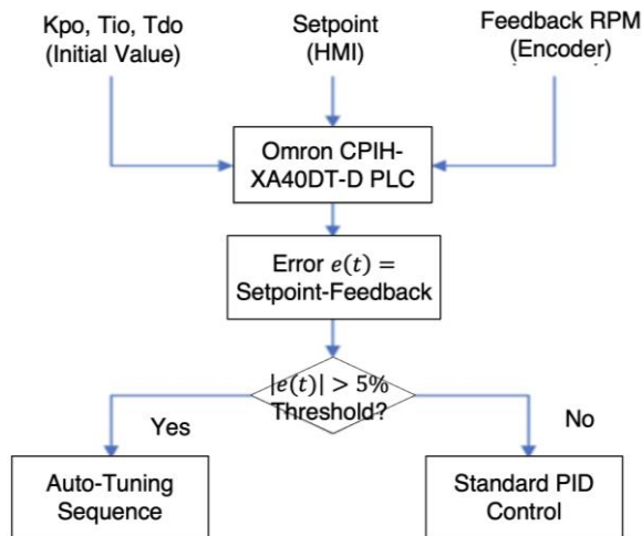
Figure 2. Flowchart of PID auto-tuning algorithm implemented on the Omron PLC.
