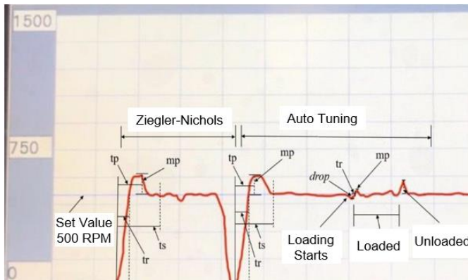
Figure 4. System response to spontaneous load disturbance at 500 RPM.
