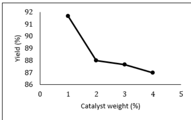
FIGURE 4. Effect of catalyst weight on biodiesel yield.
